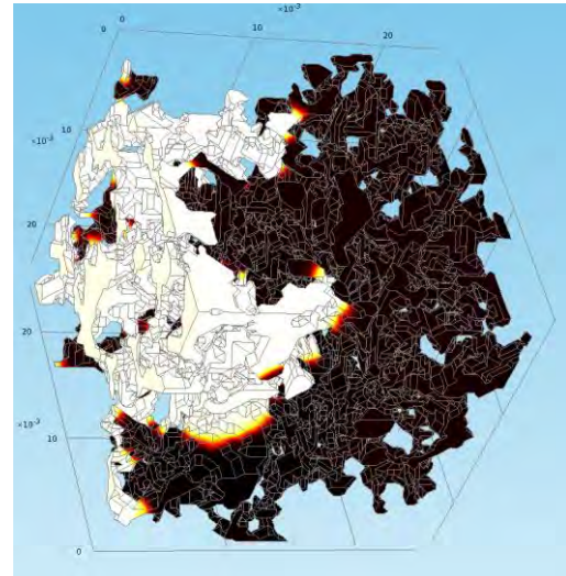
Figure 7. Two-phase flow in Bentheimer sandstone: displacement is stable as the injected (white) liquid is more viscous ( M=0.1 ) than the displaced (black) one. Flow is directed from left to right.
